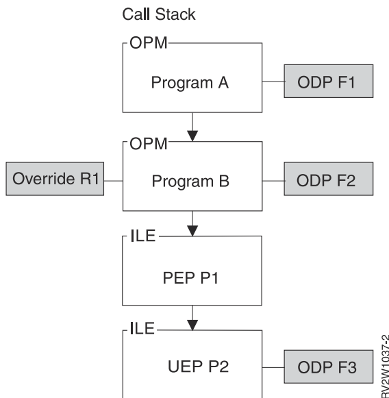
Figure 26. Call-Level Scoping
